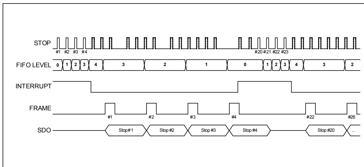
Figure 61: BLOCKWISE_FIFO_READ
