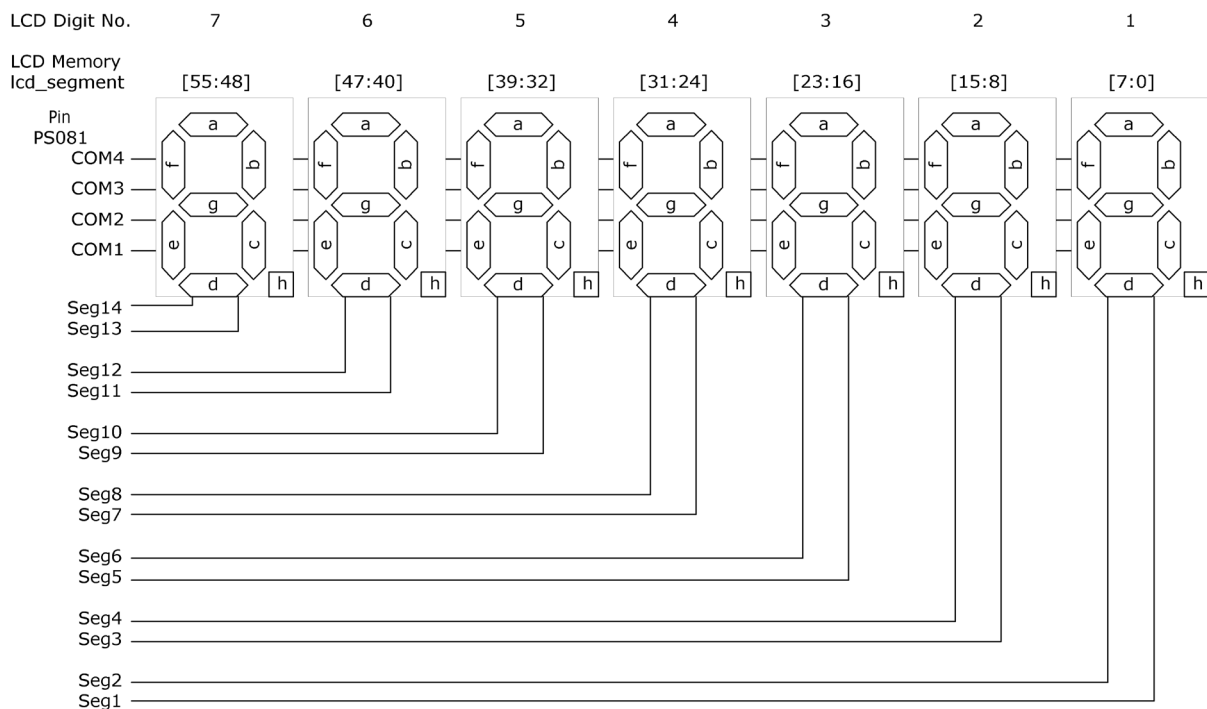
Figure 4.6 4-MUX (1/4 duty)
