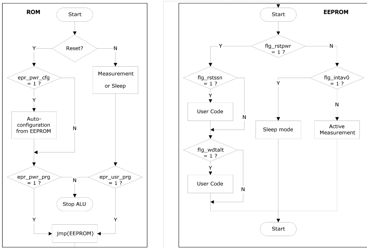
Figure 6.3 Flow chart
