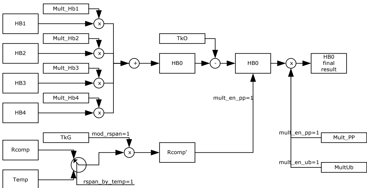
Figure 3.25 Post-processing
