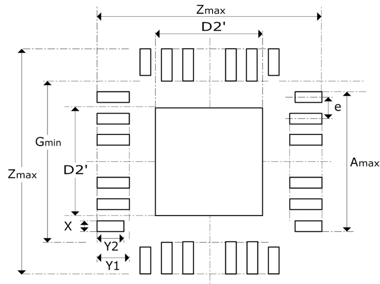
Figure 2.9 Pad Layout
