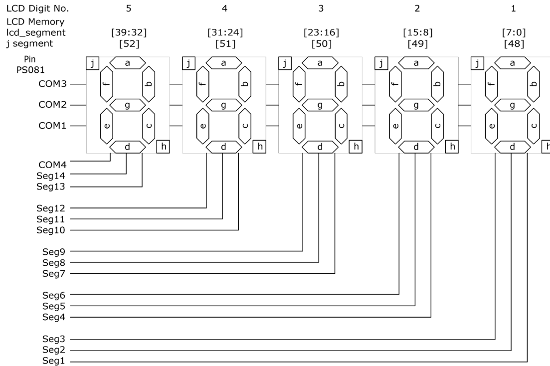
Figure 4.7 3-MUX ( 1/3 duty)
