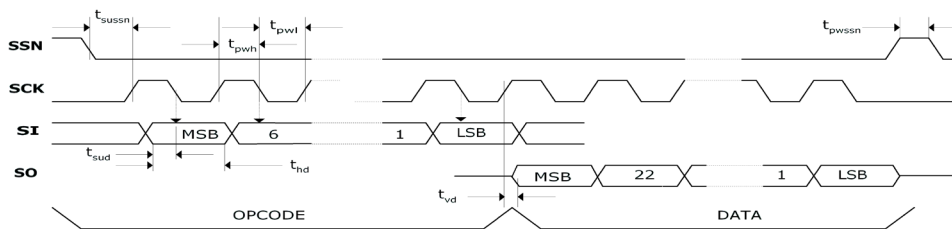
Figure 2.6 SPI-Read access
