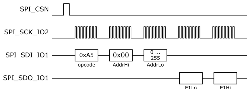
Figure 4.17 User-EEPROM read access
