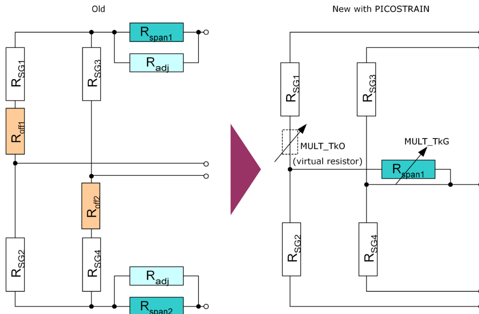
Figure 3.26 Correction of Gain and Offset Drift
