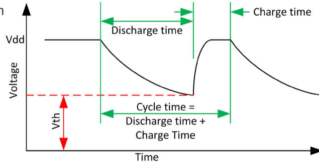
Figure 3-1 Cycle Tim
