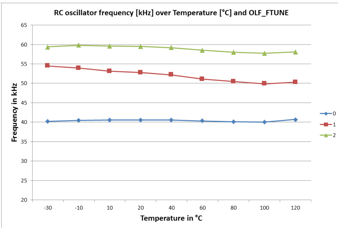
Figure 2-10: RC oscillator frequency dependence on temperature and OLF_FTUNE setting O-2
