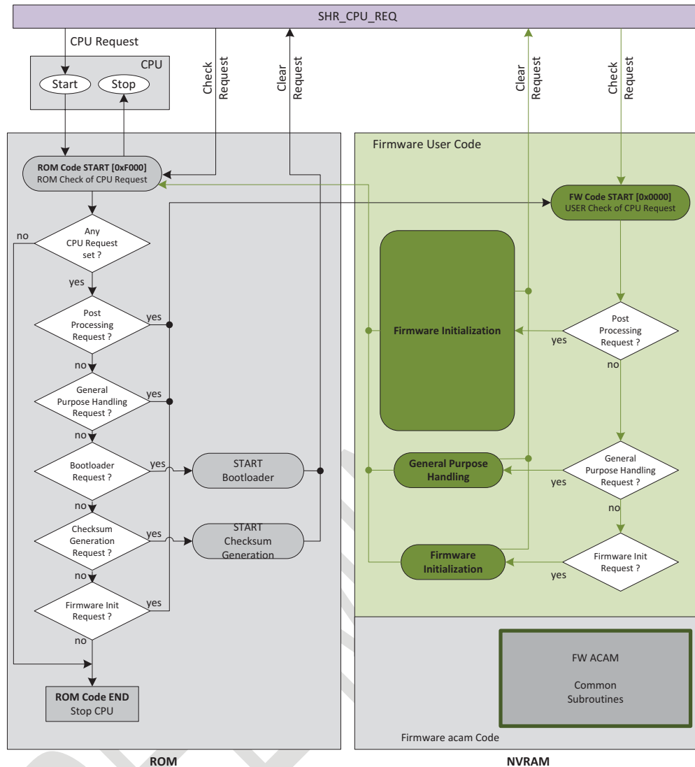
Figure 6-1 CPU request handling
