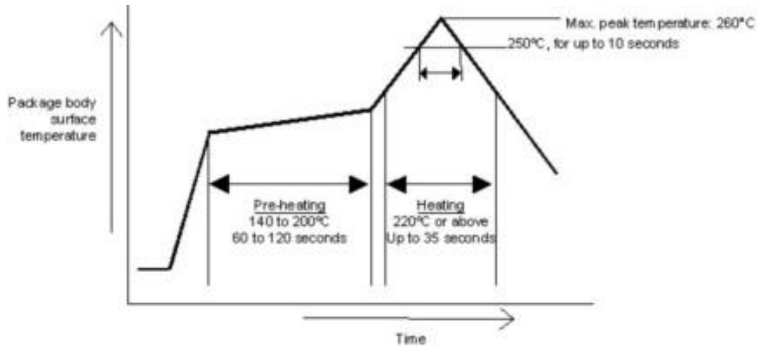
Figure 2-8: Soldering profile
