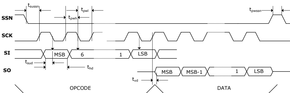
Figure 2.2: SPI Read
