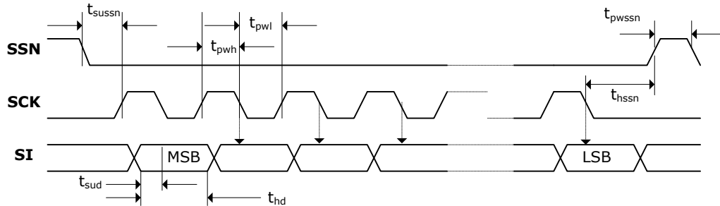
Figure 2.1: SPI Write
