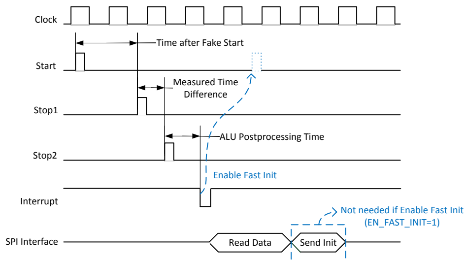
Figure 2.2 Timing – Single Measurement without Calibration
